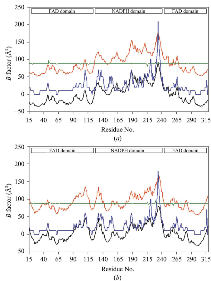
Figure 2 The plot of temperature factor along the polypeptide chain in (a) subunit A and (b) subunit B . The total B factor (red), the TLS component (black), the residual B factor (green) and the B factor from NMA (blue) are plotted. As can be seen clearly, there is a close correlation between the NMA-derived and the experimental B factors.
