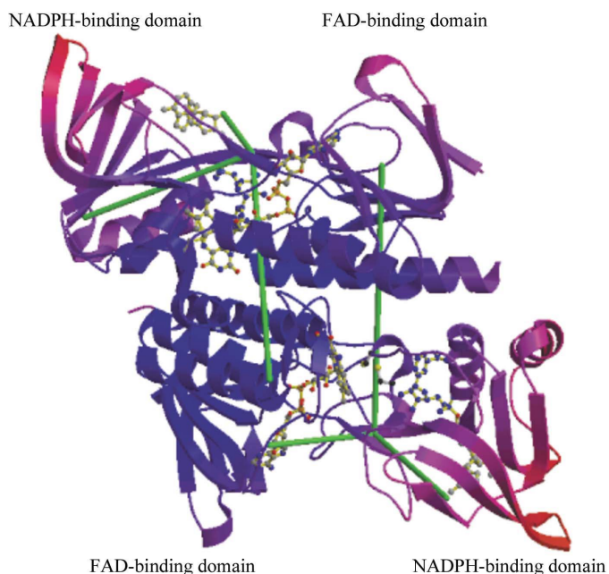
Figure 1 Overall structure of M. tuberculosis TrxR dimer. The molecule has been coloured according to the distribution of B factors, with the lowest B values being depicted in blue and the high values in red. The cofactors FAD and NADPH are shown in ball-and-stick representation. The principal axes of the libration tensor for the NADPH domains of M. tuberculosis TrxR are shown in green. Figs. 1, 3, 5 and 7 were generated using MOLSCRIPT (Kraulis, 1991) and RASTER3D (Merritt & Bacon, 1997).
