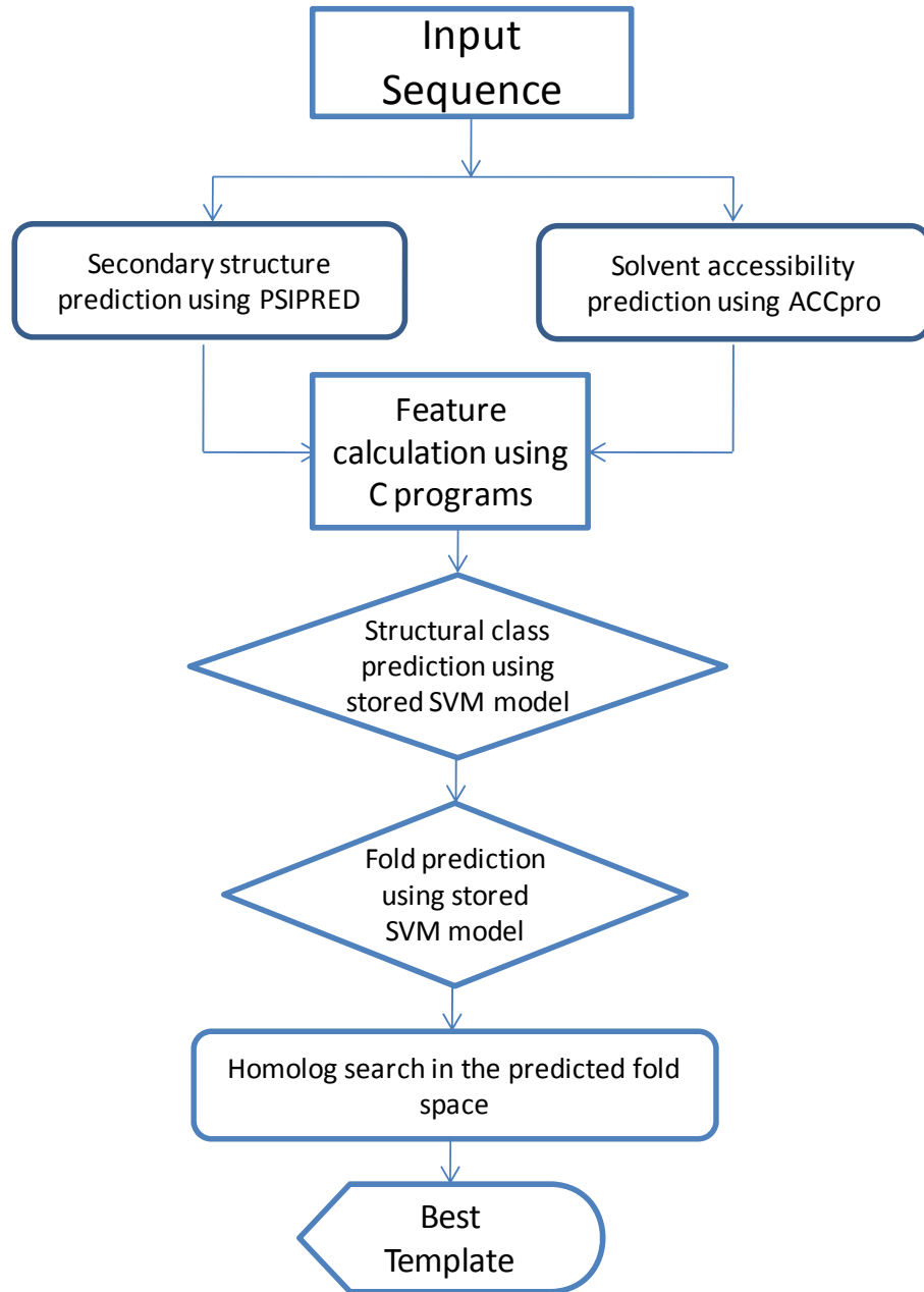
Figure 1: Outline of the steps involved in hierarchical protein fold prediction (HPFP).
